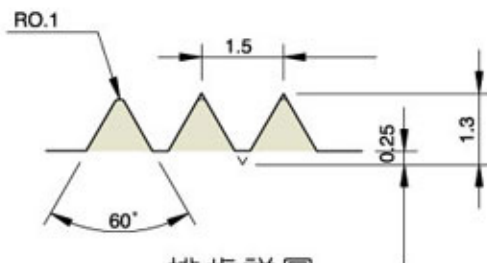
排齒詳圖 Drawing of Serration
